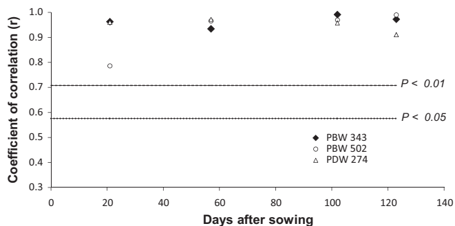
Fig. 4. Coefficients of correlation of LCC score with leaf nitrogen concentration at different growth stages in different wheat genotypes.
