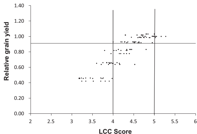
Fig. 6. Cate-Nelson graphic analysis relating LCC score of wheat leaves at different growth stages with relative grain yield.
